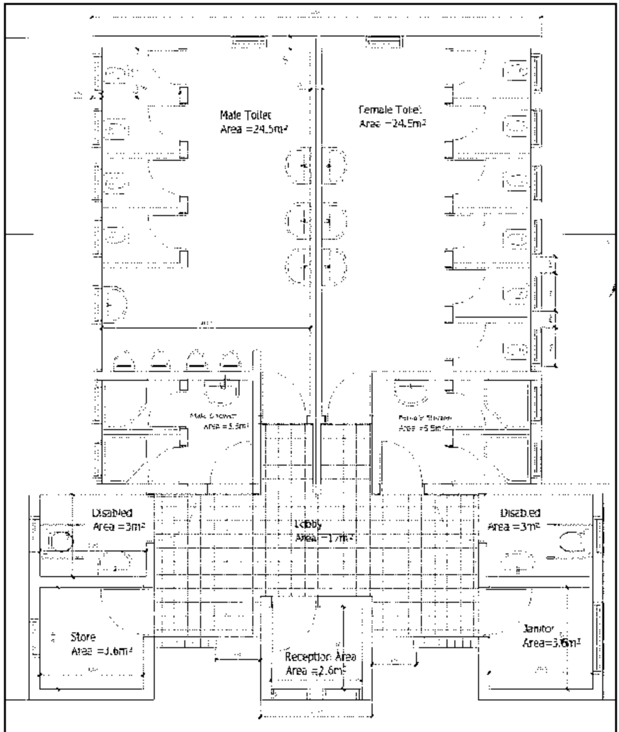
Figure 5: Typical Floor Plan for Public Toilet
